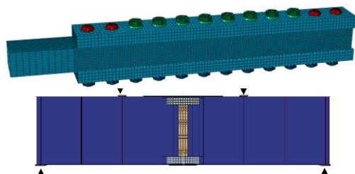
Fig.3 Finite element method model
