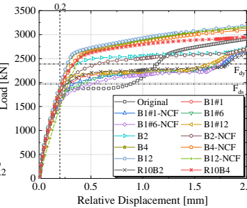
Fig.5 Relationship between load and relative displacement
