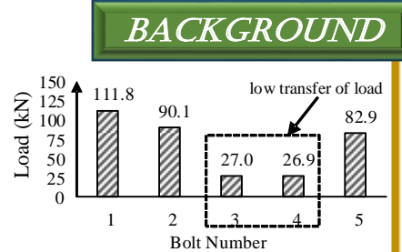
Fig.2 Load sharing of joints (when slip occurred)
