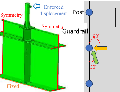
Fig.3 Analysis model and boundary conditions
