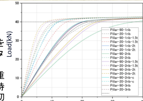
Fig.5 Load-displacement relationship
