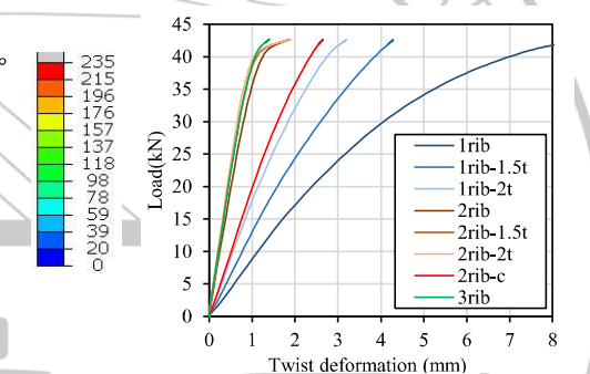
Fig.6 Load-twist deformation relationship
