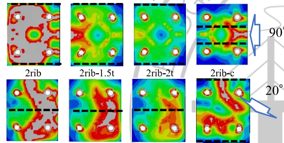
Fig.7 Mises stress contour diagram for Base-Plate at design load
