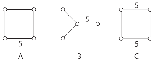
FIGURE 9. The three Coxeter graphs of the hyperbolic Coxeter simplex of dimension 3 which describe the figures of three types of orthogonal facets of T
