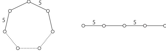
FIGURE 1. The Coxeter graphs of the compact truncated Coxeter 4-simplex and its underlying extended 4-simplex
