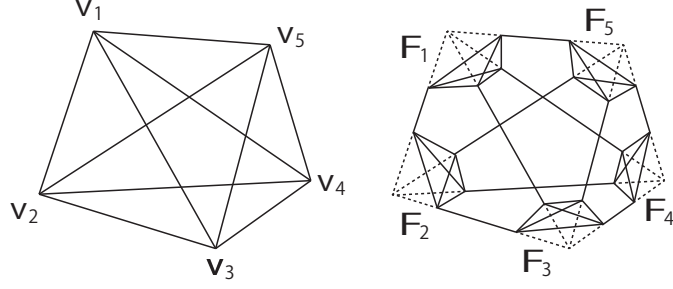
FIGURE 7. The passage to the compact totally truncated Coxeter 4-simplex T where each ultraideal vertex v_i is replaced by the orthogonal facet F_i
