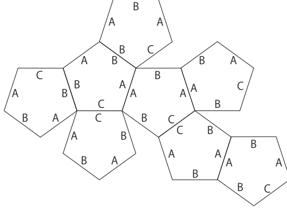
FIGURE 10. The image of the Coxeter polytope obtained by 7-times gluing of T satisfying (\ell, m, n) = (3, 2, 7)
