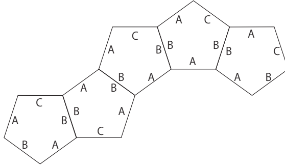
FIGURE 11. The image of the Coxeter polytope obtained by 5-times gluing of T satisfying (\ell, m, n) = (0, 5, 5)
