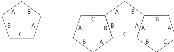
FIGURE 3. The images of a Coxeter domino T and Coxeter dominoes
