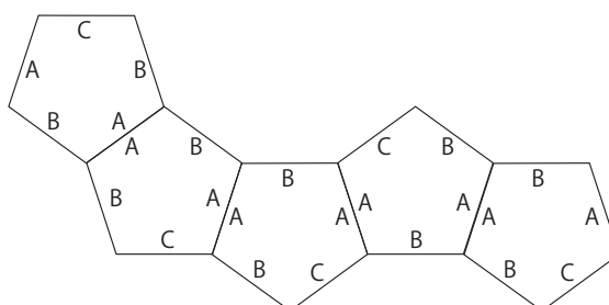
FIGURE 12. The image of the Coxeter polytope obtained by 5-times gluing of T satisfying (\ell, m, n) = (5, 0, 5)
