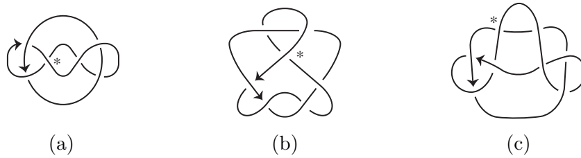
FIGURE 5. (a) T'_4 \rightarrow T_4! , (b) T_6 \rightarrow 6^2_2 , (c) 6^2_3 \rightarrow T_6 .
